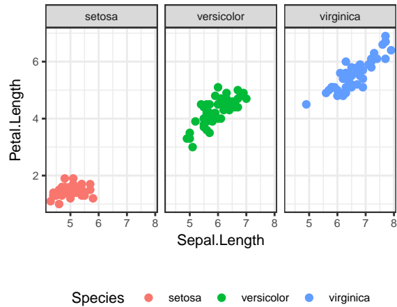
Figure 1: iris data
