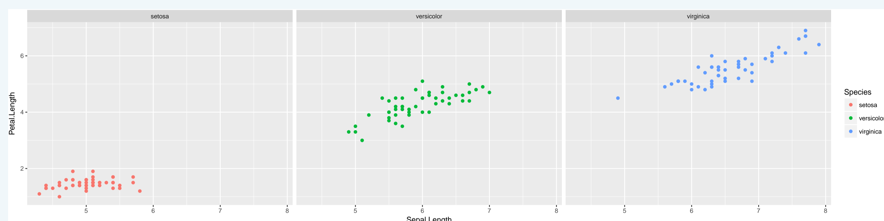
Figure 2: iris data
